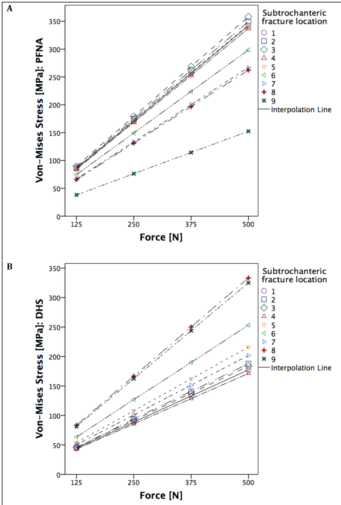
Supplementary Figure 1: Scatter plots linear relationship between force and von-Mises stress for (A) PFNA and (B) DHS implants. Hence: STF location is based on fracture distance below LT in steps of 5 mm (e.g. location 1 is 0.5 cm and location 9 is 4.5 cm below LT). Abbreviation: STF (Subtrochanteric fracture), MPa (Megapascal), N (Newton), PFNA (Proximal Femoral Nail Antitrotation), DHS (Dynamic Hip Screw) and LT (Lesser Trochanter).
